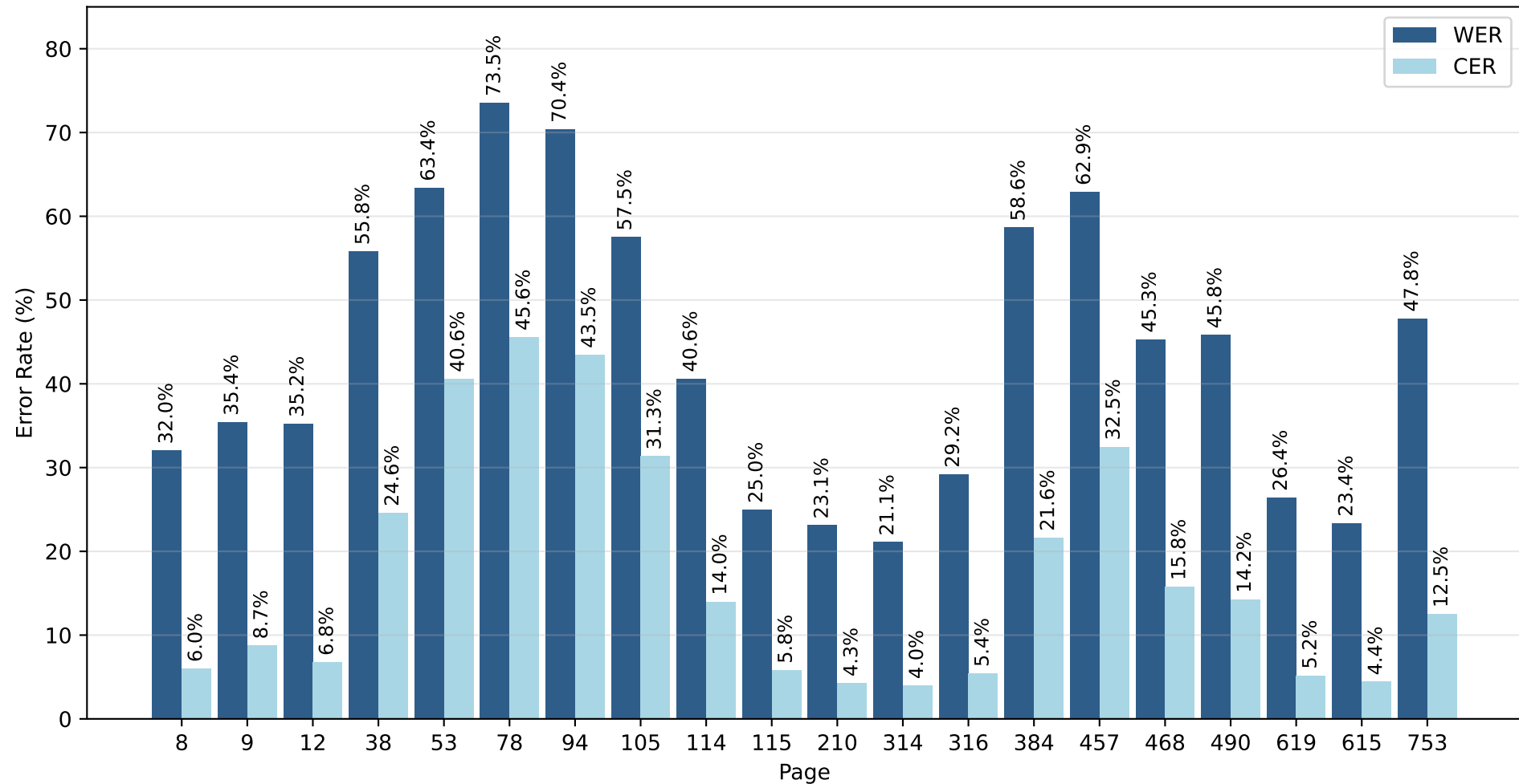
Experiment 2 - Pytesseract
