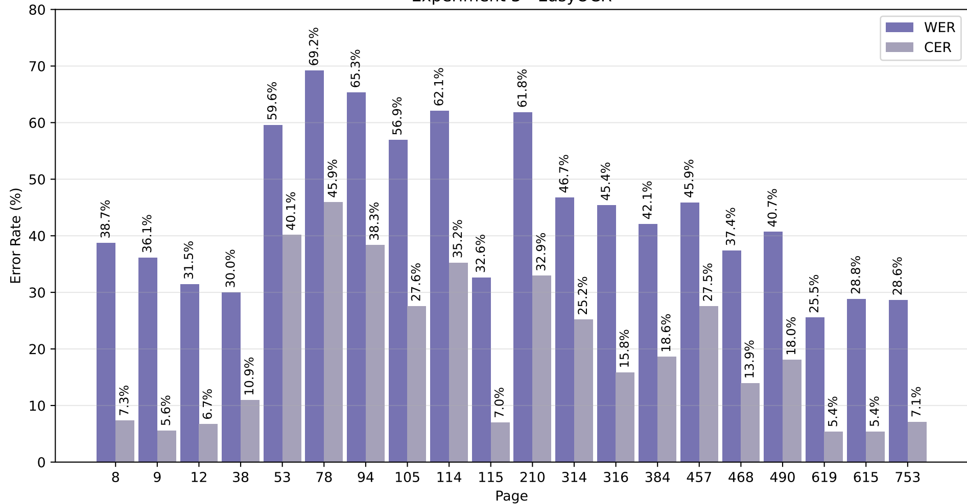
Experiment 3 - EasyOCR
