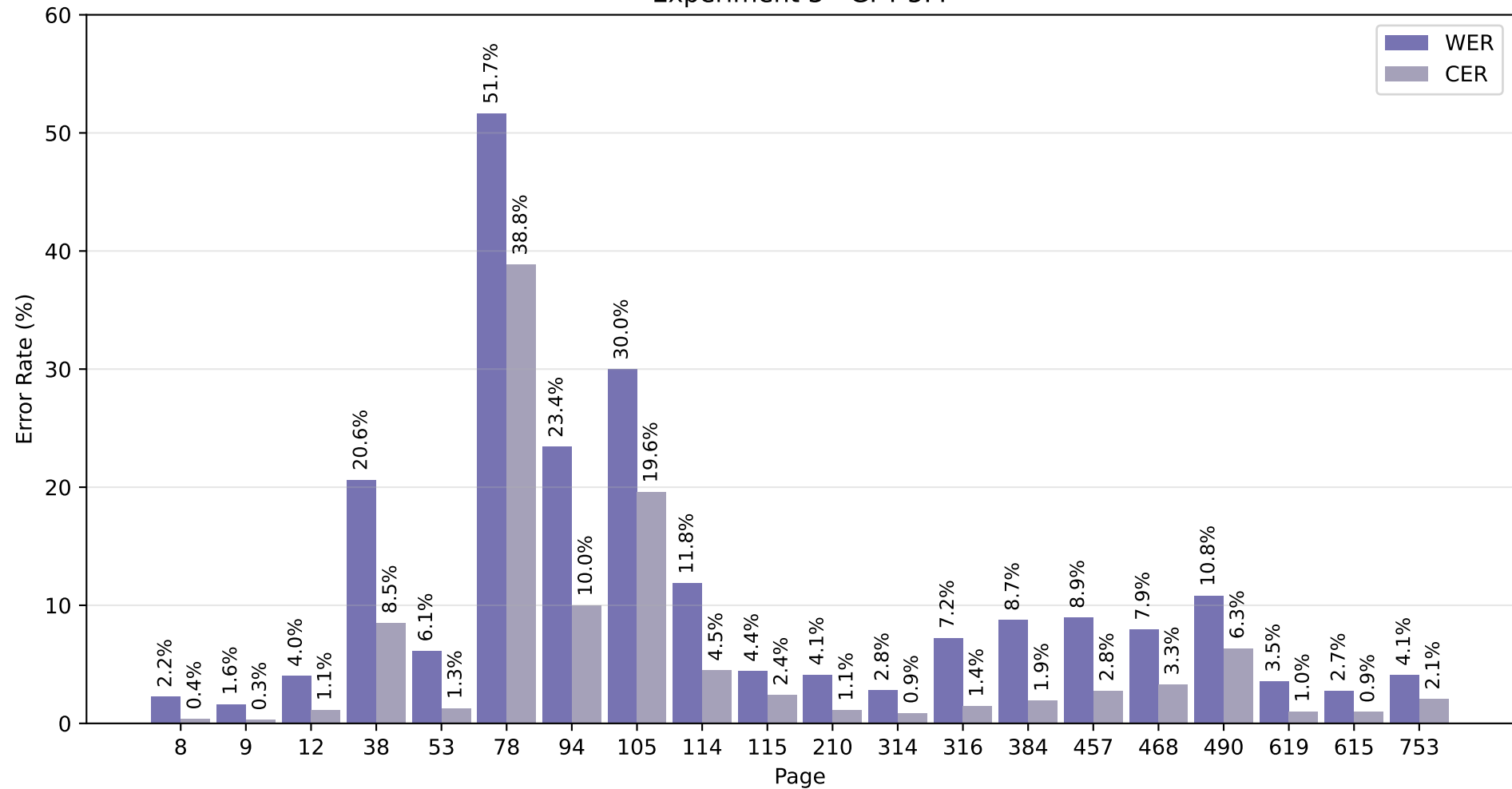
Experiment 3 - GPT-5.4
