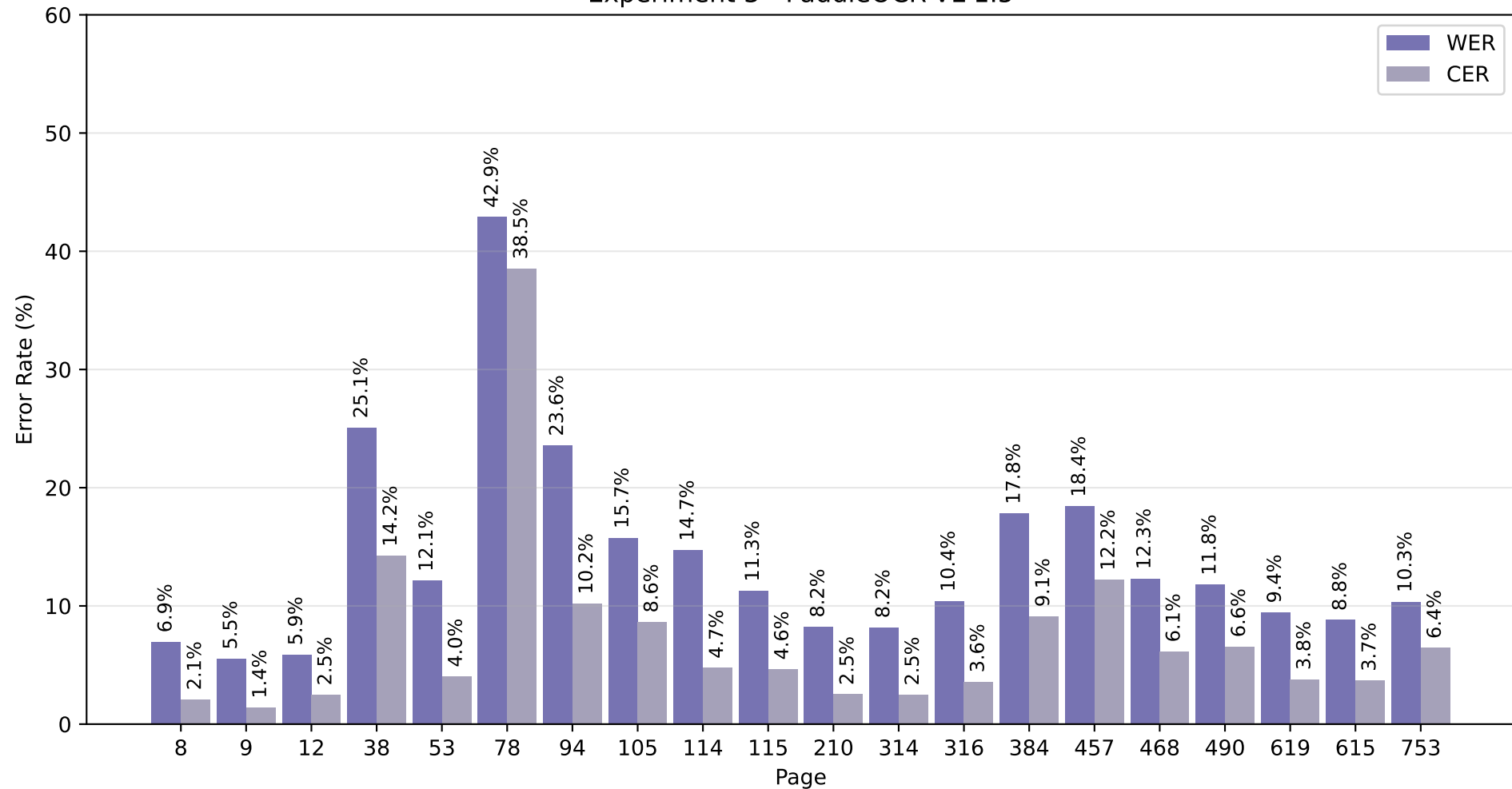
Experiment 3 - PaddleOCR-VL 1.5
