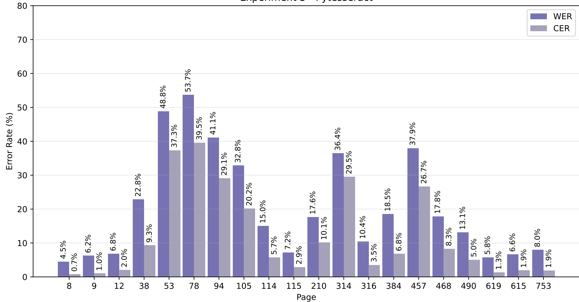
Experiment 3 - Pytesseract
