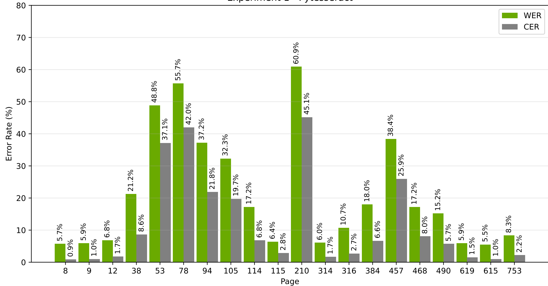
Experiment 1 - Pytesseract
