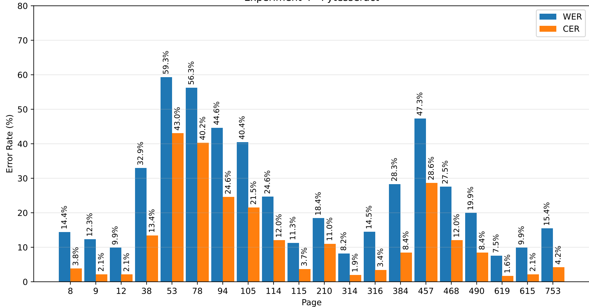
Experiment 4 - Pytesseract
