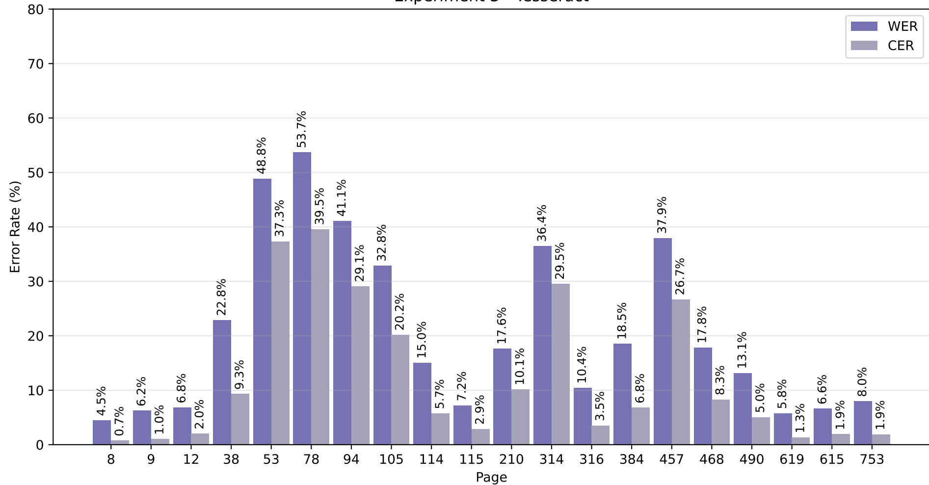
Experiment 3 - Tesseract
