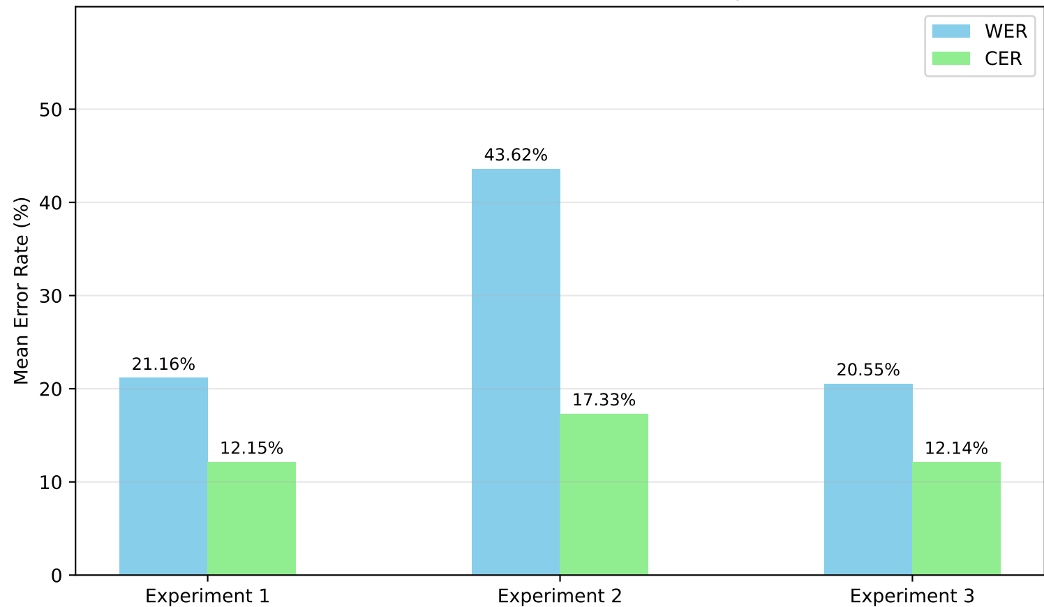
Tesseract - Mean WER and CER Across Experiments
