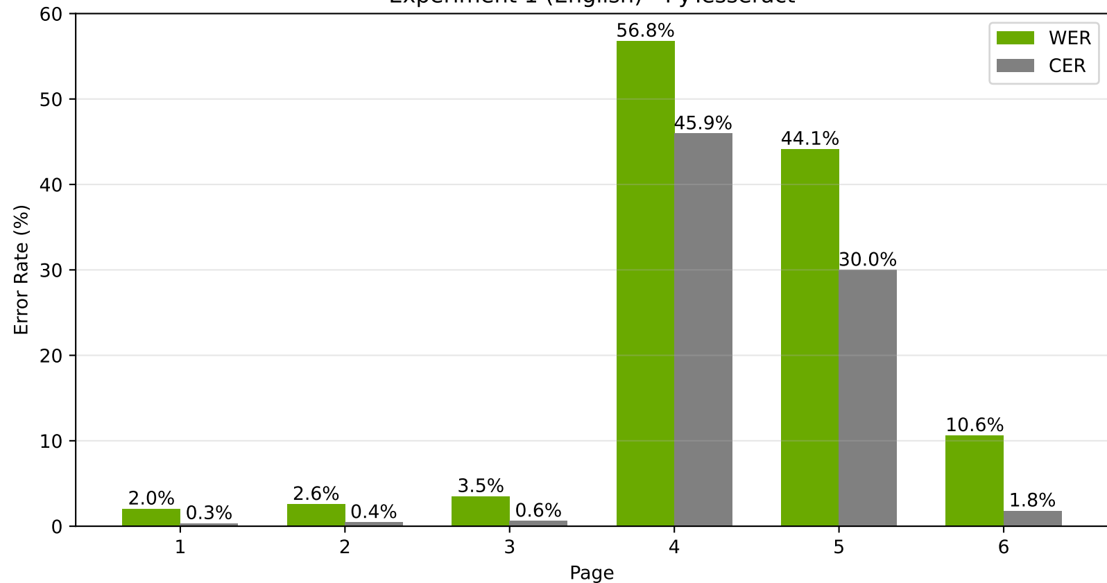
Experiment 1 (English) - PyTesseract
