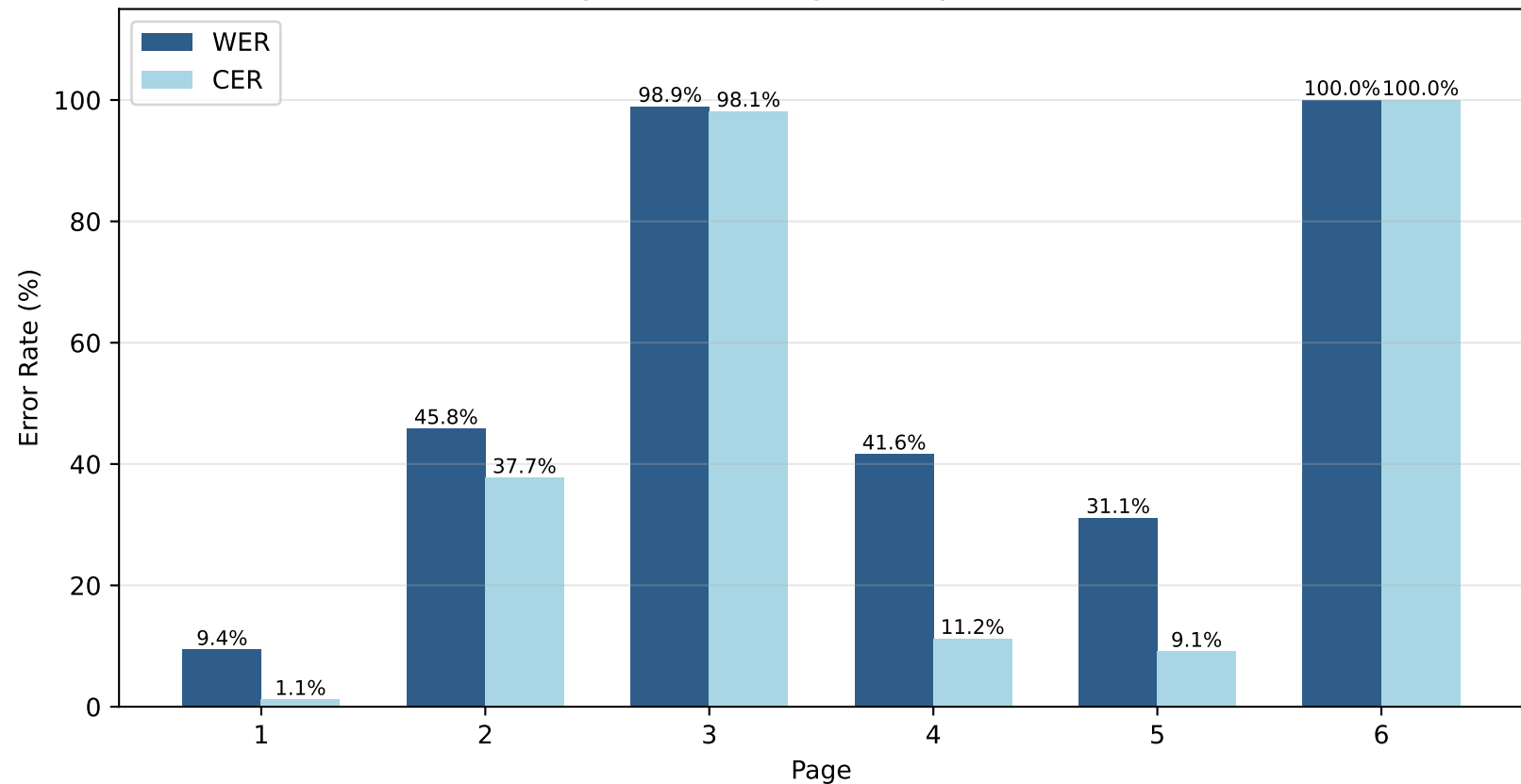
Experiment 2 (English) - PyTesseract
