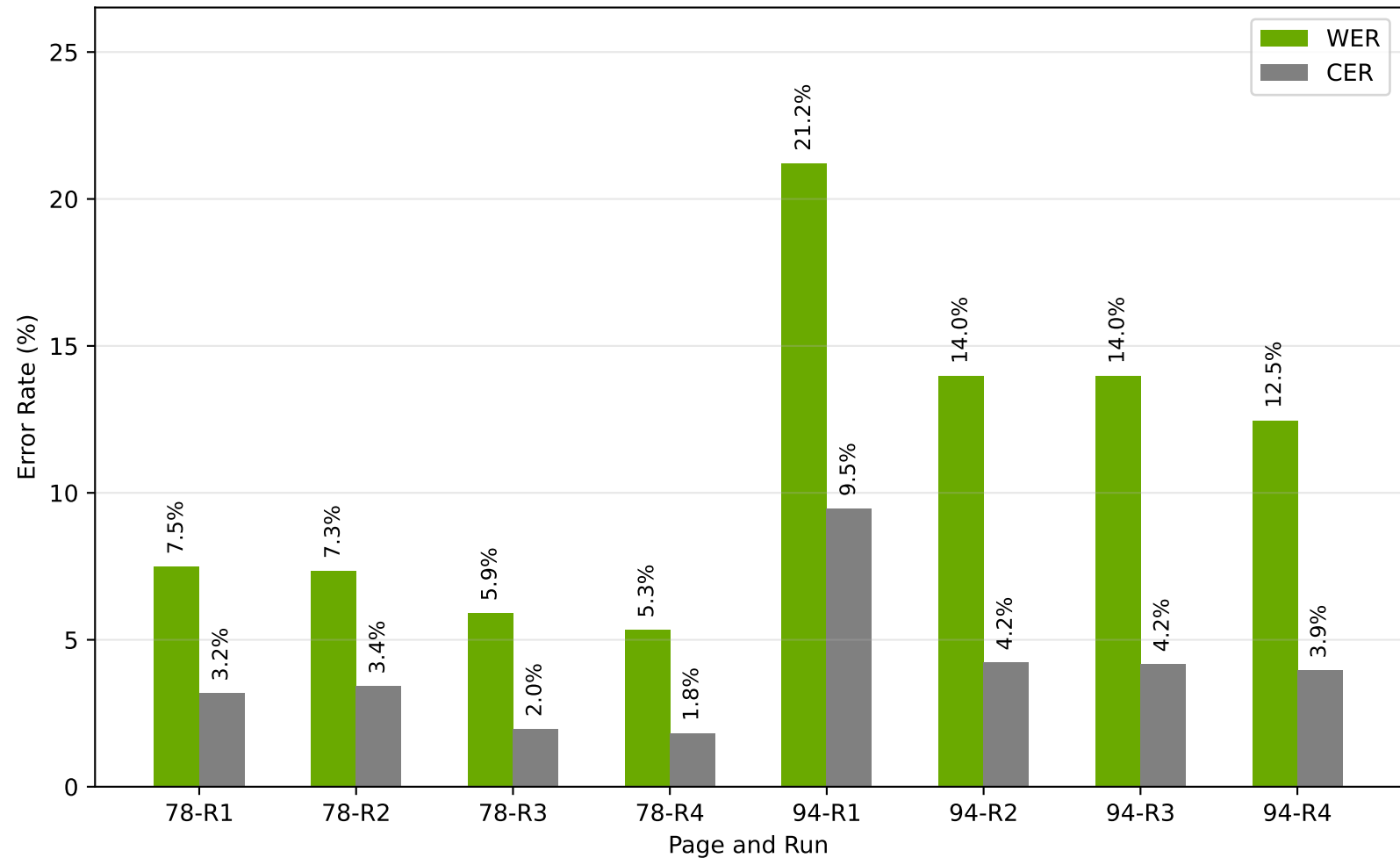
Recognition Improvement - Gemini 3.1 Pro
