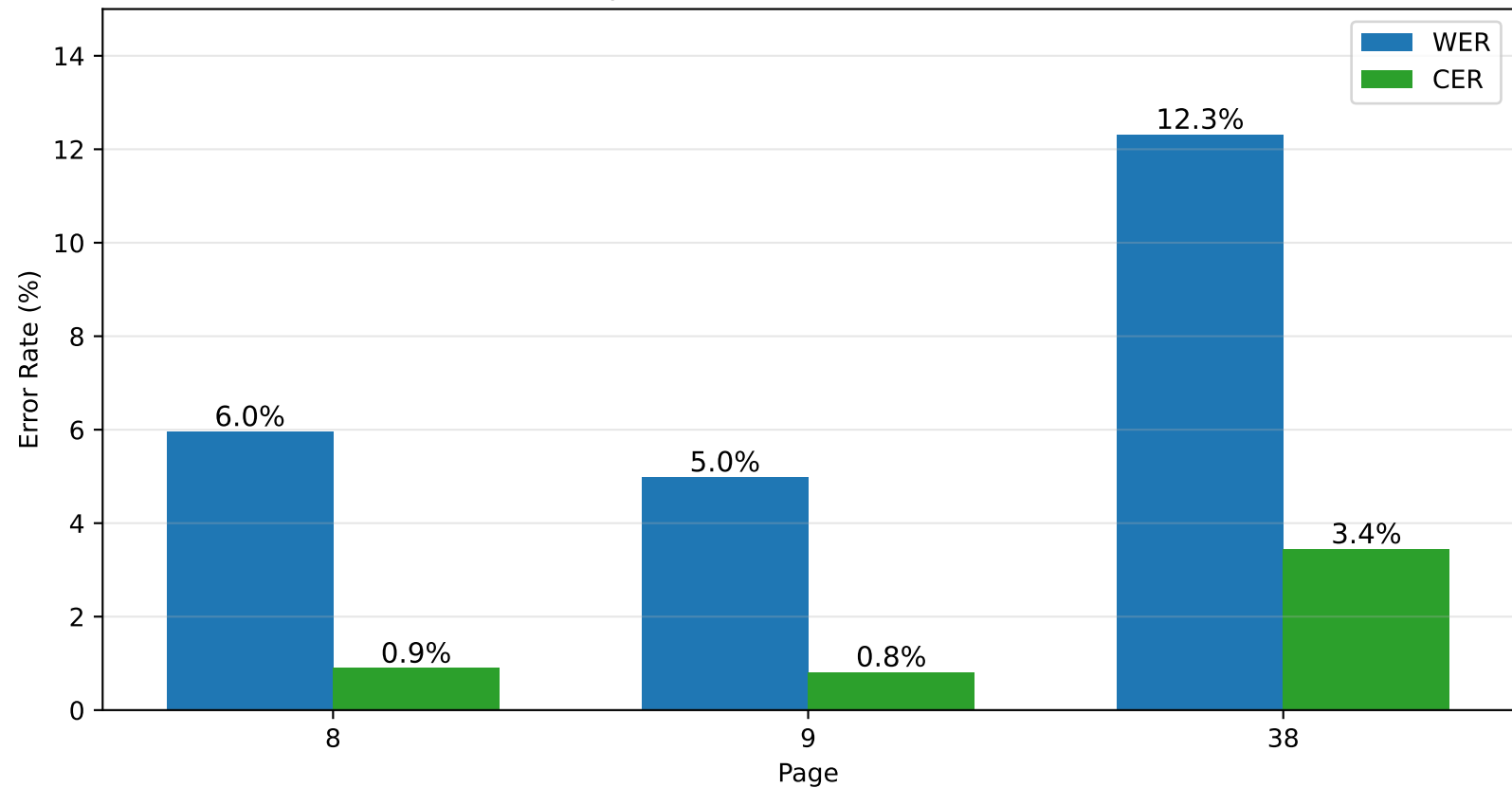
Prompt-2 Results: Qwen3.5-35B-A3B
