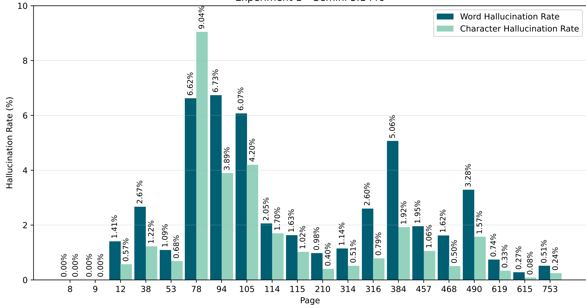
Experiment 1 - Gemini 3.1 Pro
