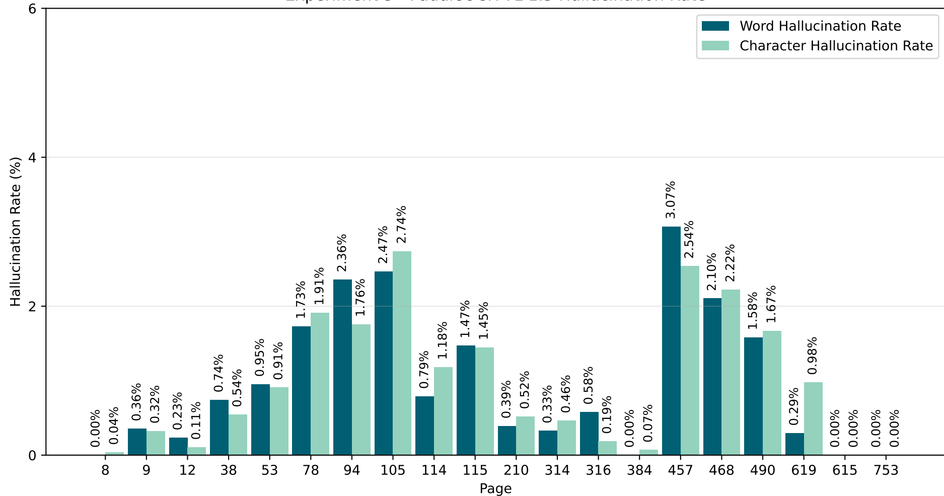
Experiment 3 - PaddleOCR-VL 1.5 Hallucination Rate
