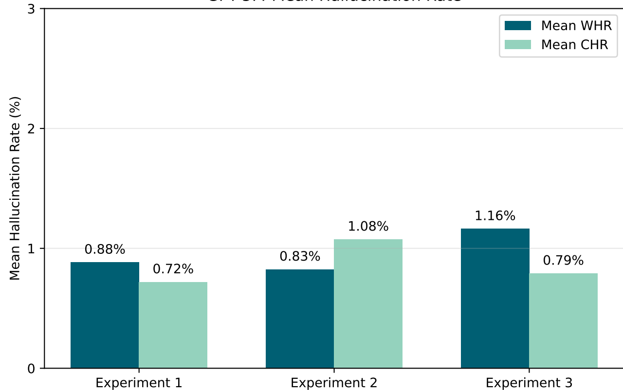
GPT-5.4 Mean Hallucination Rate
