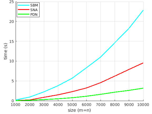
Figure 2. Time versus dimension, SBM (cyan), SNA (red), PDN (green). PDN grows slowest compared to SBM and SNA.
