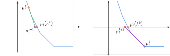
Figure 1. Primal update scheme
