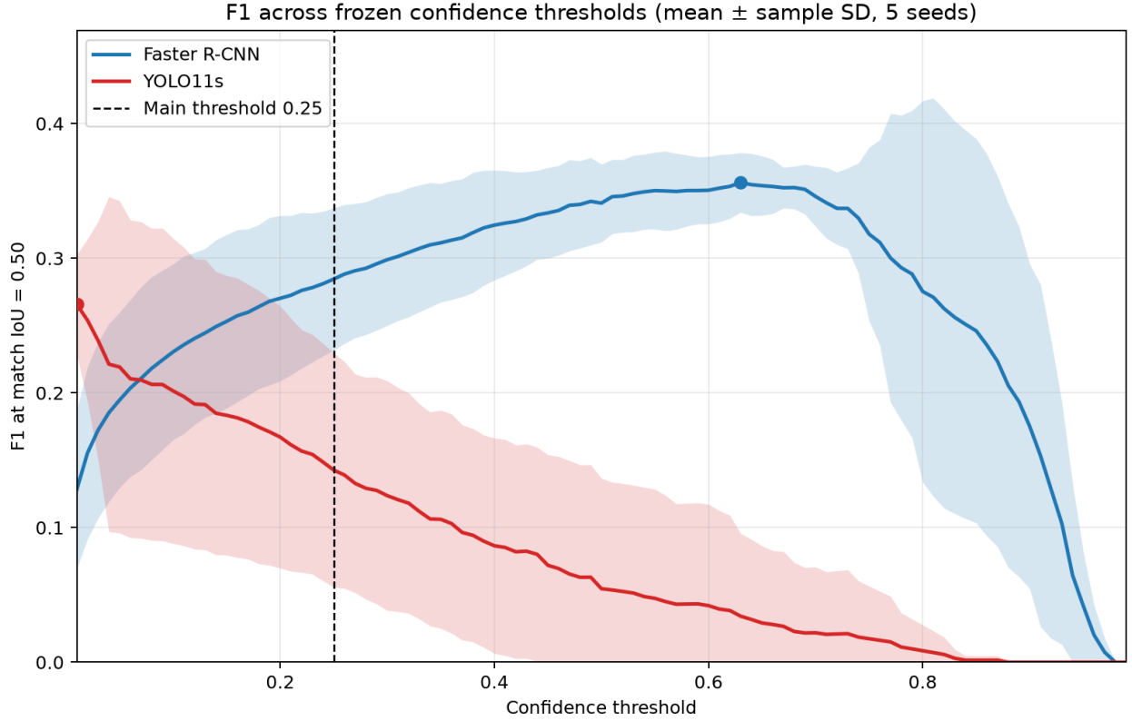
Figure 1b. Exploratory five-run F1 versus raw threshold. Test-set maxima are descriptive and were not used for threshold selection.
