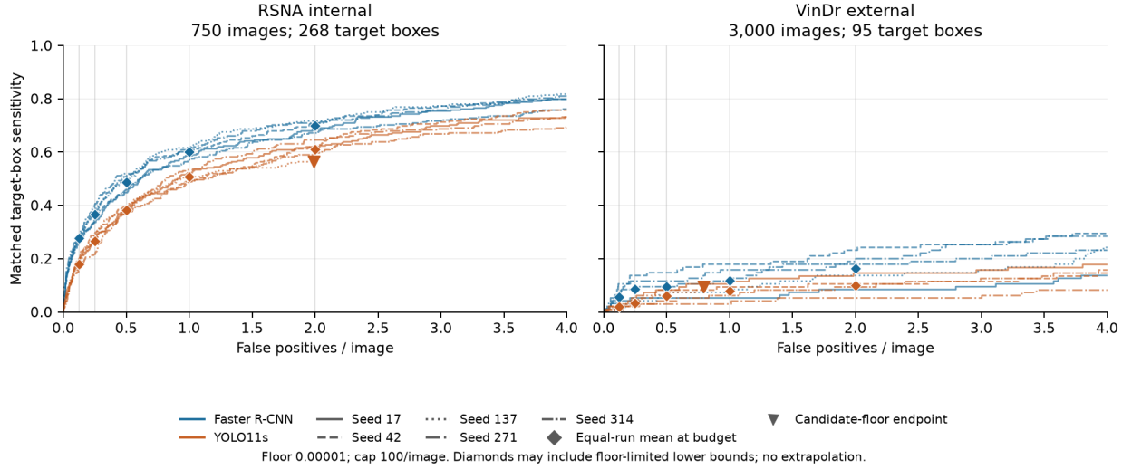
Figure 2. Internal and external observed exact-score FROC, with all five runs and their candidate-floor endpoints. Curves have finite retained support at floor 0.00001 and cap 100. External YOLO11s seed 137 is floor-limited at 1 and 2 FP/image, where the missing-support bound permits reversal. Faster R-CNN cap saturation further limits support; no unrestricted frontier ordering is established.
