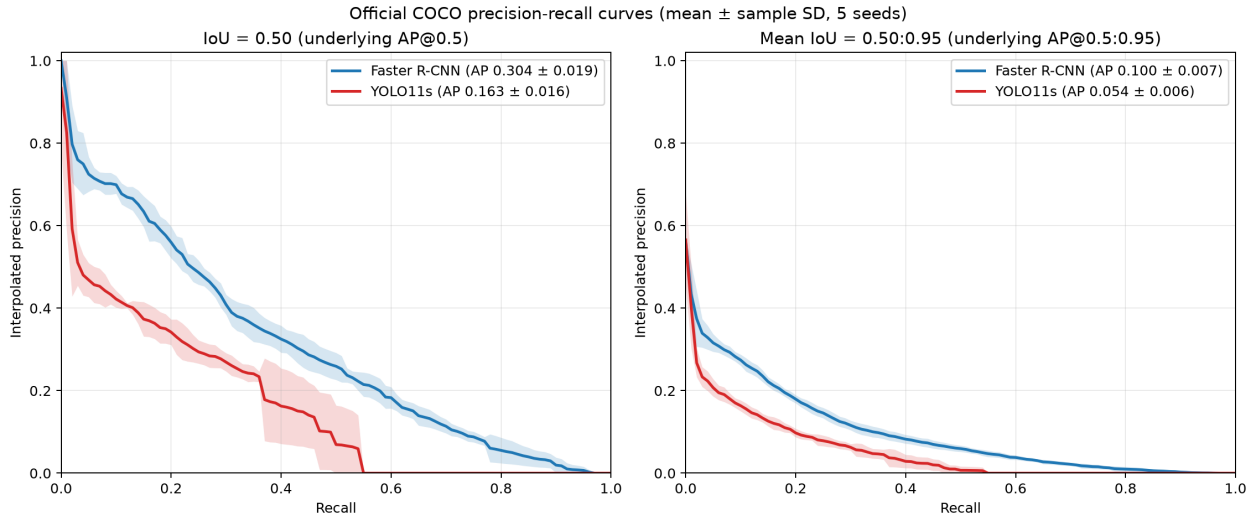
Figure 1a. Official five-run PR curves. Lines and bands show equal-run mean and sample SD, including the low-score YOLO11s run.
