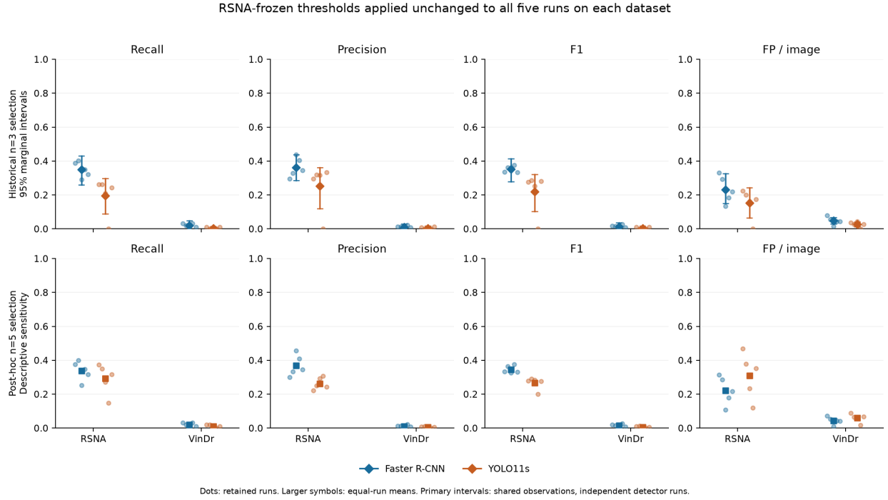
Figure 4. Transport of the frozen historical thresholds, with all retained runs and marginal training-procedure intervals; the separately labeled n=5 validation policy is descriptive post-hoc sensitivity. No VinDr threshold was selected.
