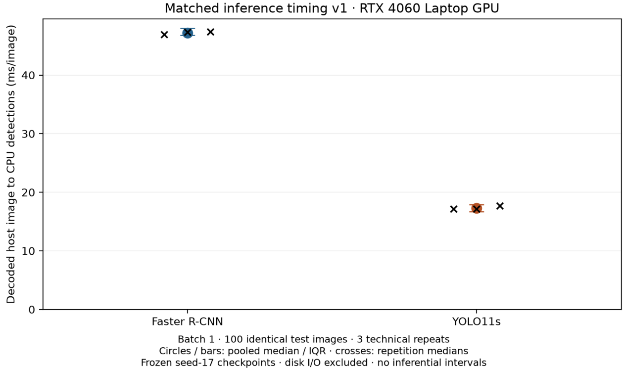
Figure 3. Matched decoded-host inference timing on the reporting laptop. Three repetitions per primary checkpoint are technical measurements; latency dispersion is not training-run uncertainty.
