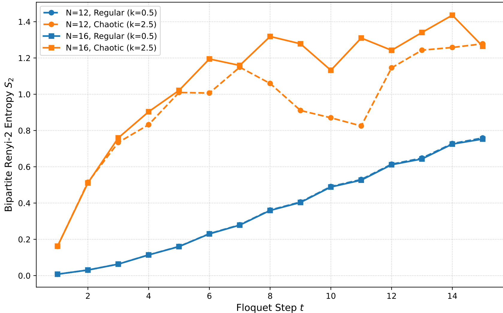
Finite-Size Scaling of Entanglement Entropy (MPS, \chi = 256 )
