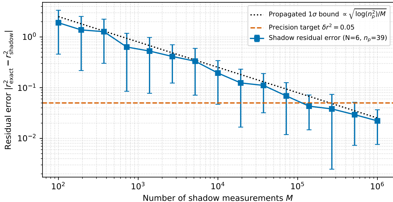
Classical-shadow convergence — N=6 , D=3
