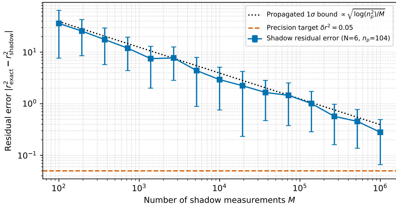
Classical-shadow convergence — N=6 , D=8
