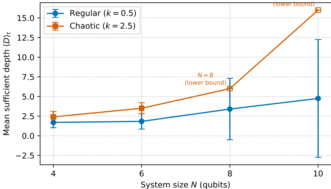
Mean circuit depth required vs. system size (direct optimization, averaged over Floquet steps)
