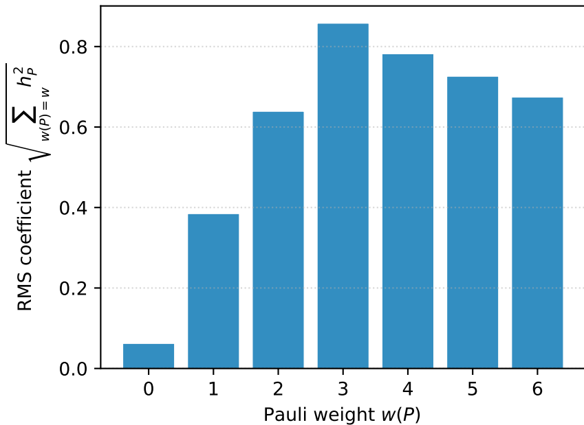
Pauli-weight distribution of H ( N = 6, k = 2.5 )
