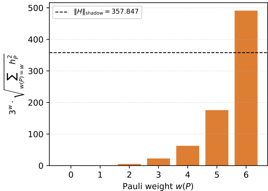
Shadow-norm contribution per weight ( N = 6 )
