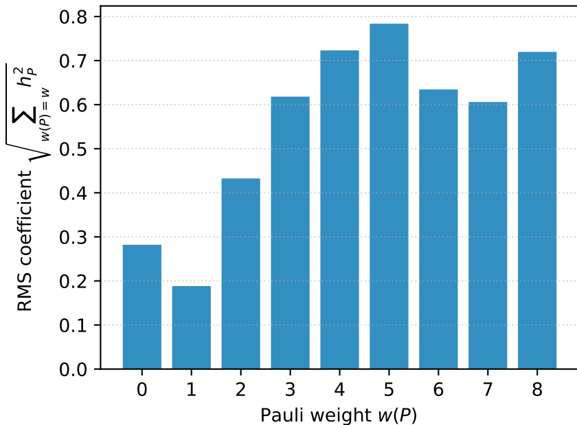
Pauli-weight distribution of H ( N = 8, k = 2.5 )
