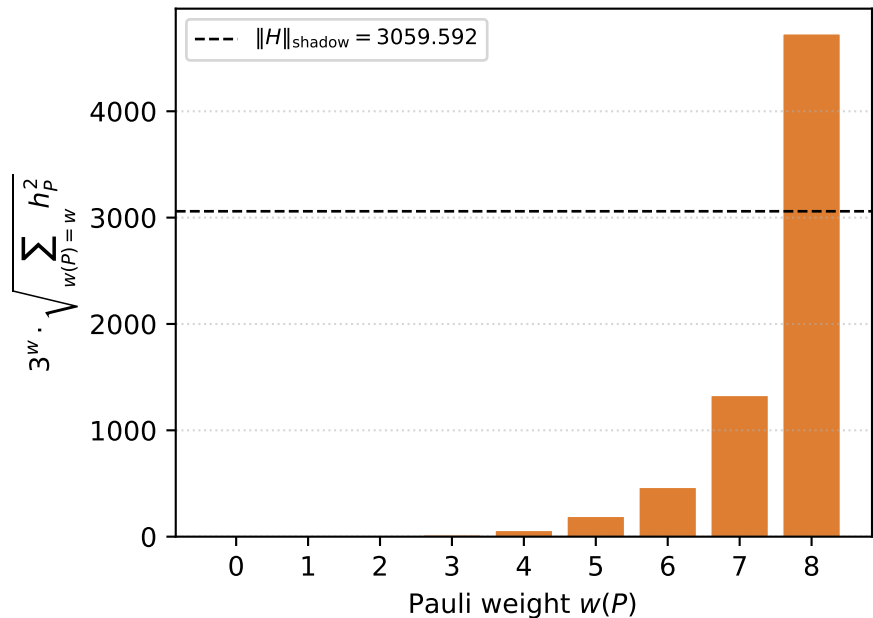
Shadow-norm contribution per weight ( N = 8 )
