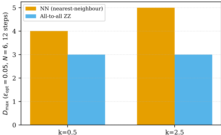
Architecture test: NN vs all-to-all entangler
