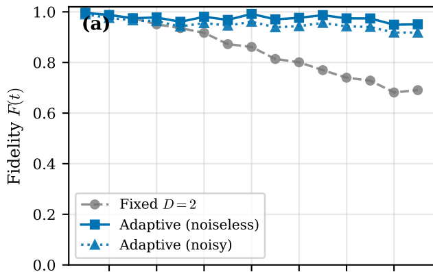
Chaotic ( k = 2.5 )
