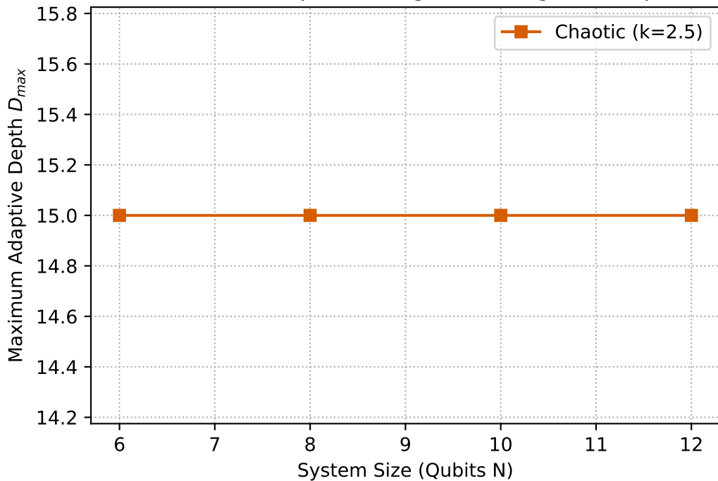
Exact VQS Depth Scaling (Resolving MPS Gap)
