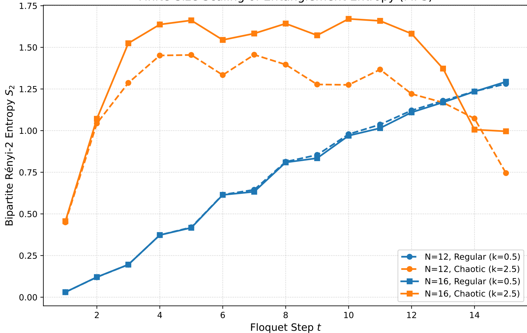
Finite-Size Scaling of Entanglement Entropy (MPS)
