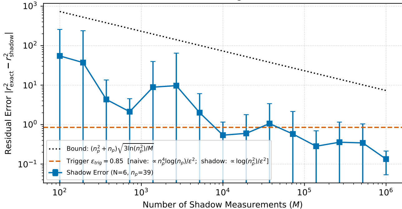
Classical Shadow Convergence — N=6, D=3
