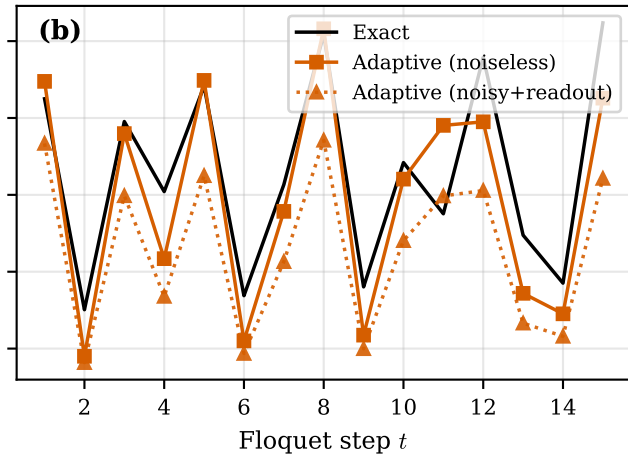
Chaotic ( k = 2.5 )
