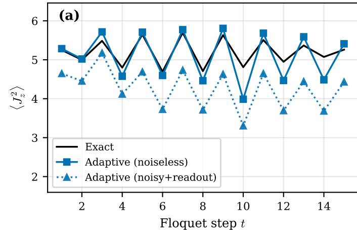
Regular ( k = 0.5 )
