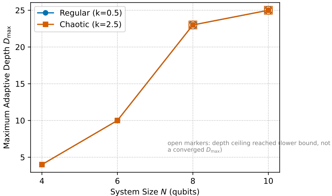
D_{\max} vs. System Size (depth ceiling = N + 15 )
