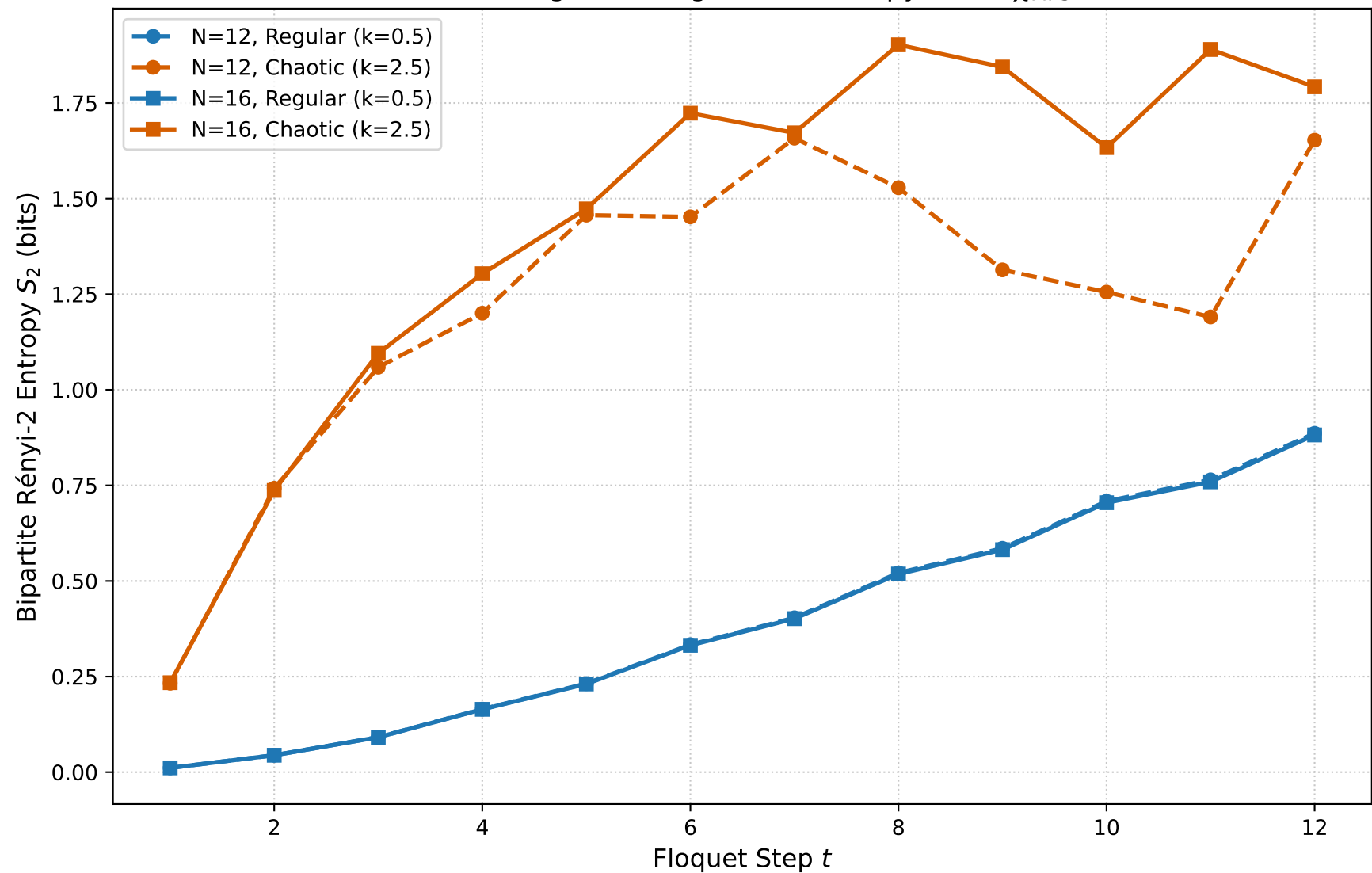
Finite-Size Scaling of Entanglement Entropy (MPS, \chi_{\text{MPS}} = 256 )
