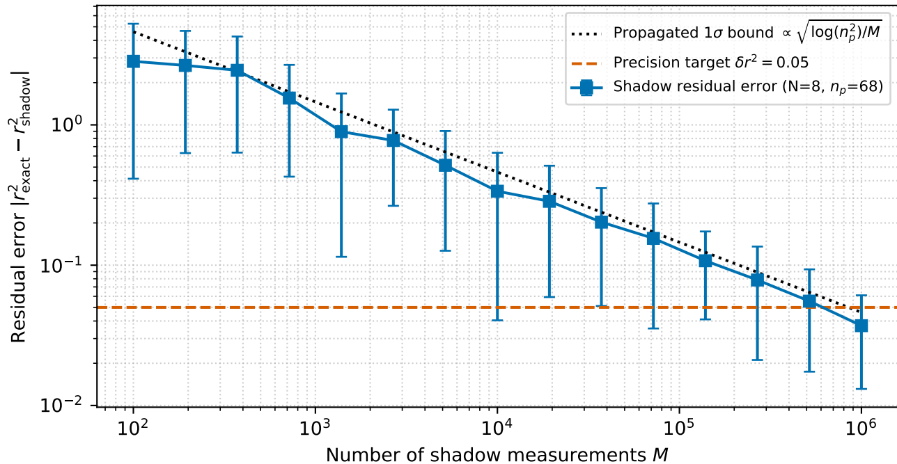
Classical-shadow convergence — N=8 , D=4
