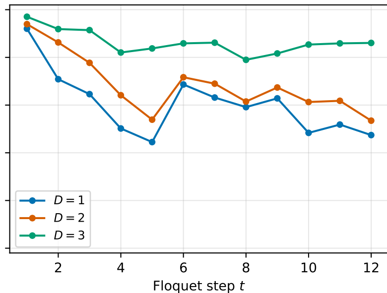
(b) Chaotic ( k = 2.5 )
