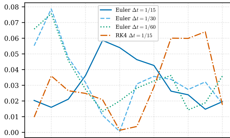
Regular — Residual r^2 at D = 1
