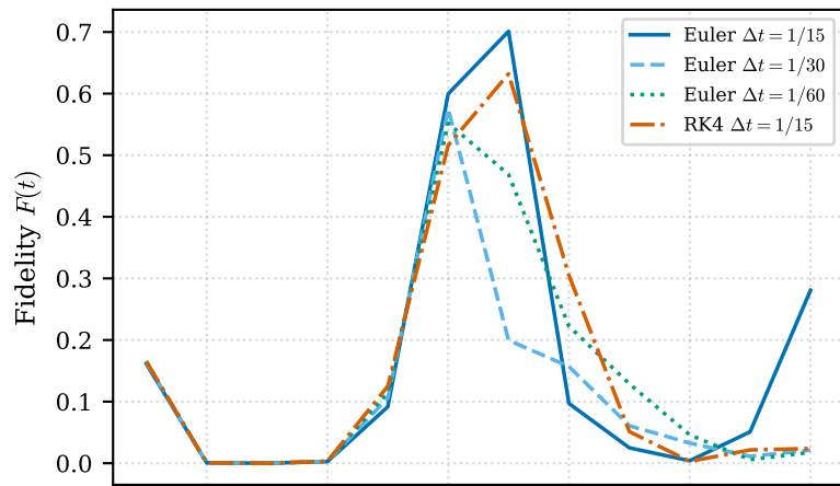
Chaotic ( k = 2.5 ) — Fidelity
