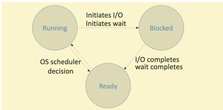
Thread state diagram
