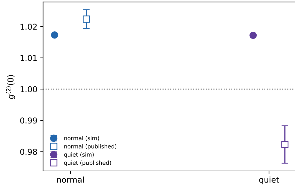
I = 4 I_{th} : sim (filled) vs Zhao et al. (open)
