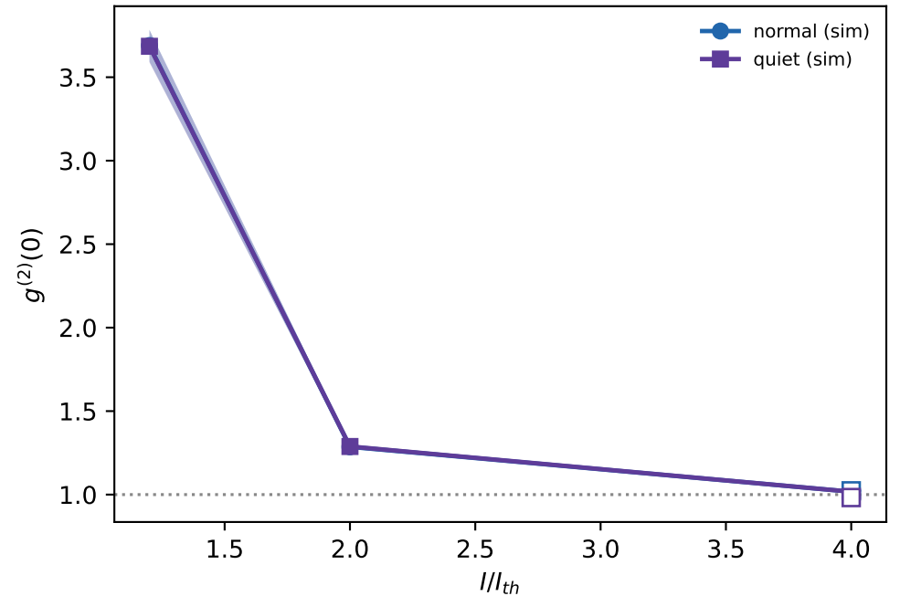
g^{(2)}(0) vs pump strength ( I_{th} raw axis = 1.050)
