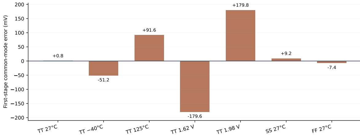
Figure 5: First-stage common-mode error across the seven simulated process, supply, and temperature conditions. Values are extracted from the supplied simulation screenshots.
