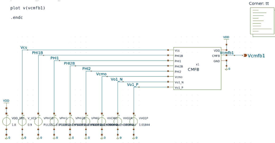
Figure 3: Standalone SC-CMFB testbench showing the four clock inputs, reference sources, sensed first-stage voltage sources, and control output.
