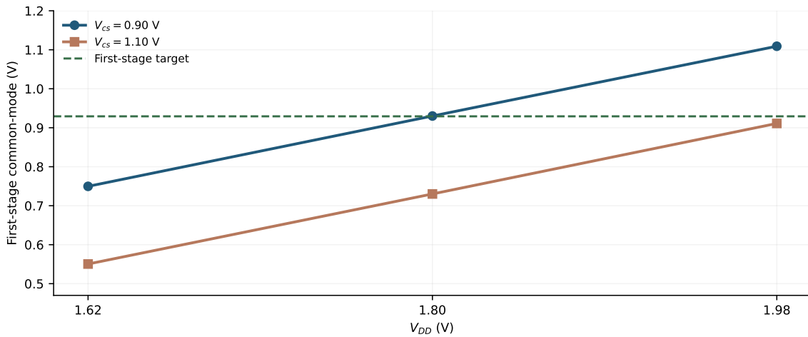
Figure 6: Shift in first-stage common mode when V_{cs} is increased from 0.90 V to 1.10 V; each marker corresponds to a measured endpoint, not to a full fitted transfer curve.
