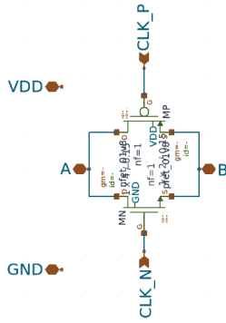
(a) Transistor-level TG cell.
