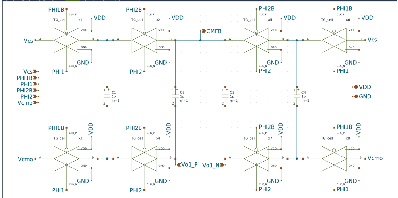
Figure 2: Implemented eight-TG / four-capacitor SC-CMFB schematic (Xschem). The left and right halves sample and redistribute charge from the two OTA first-stage outputs.
