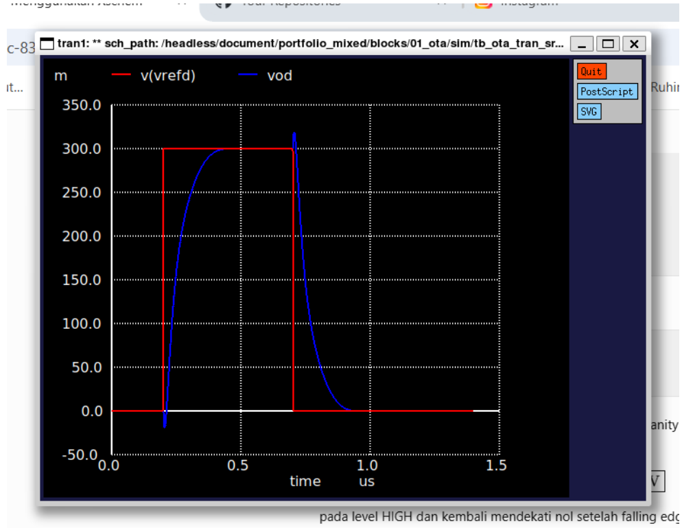
Figure 4: Large-signal differential response used for slew-rate characterization.
