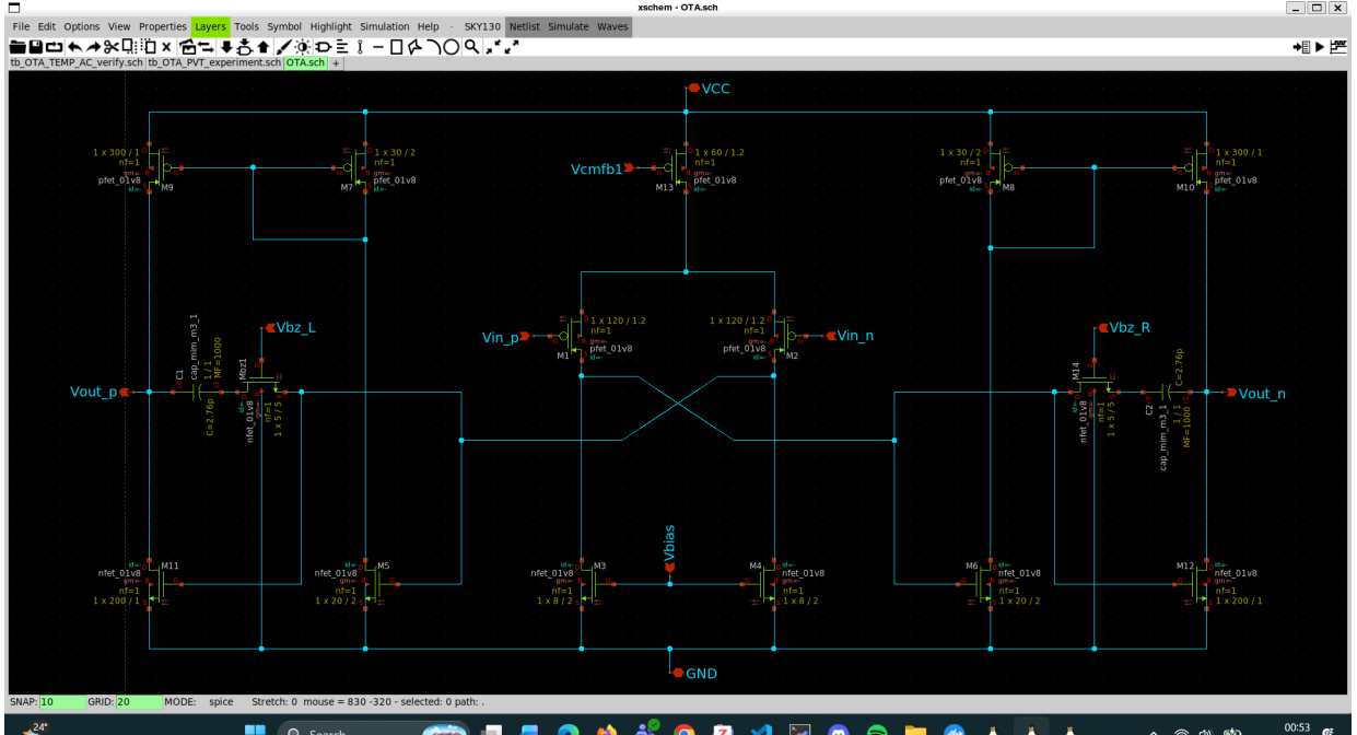
Figure 1: Initial baseline OTA schematic in Xschem before the direct-C compensation simplification. The V_{bz} -controlled branches and the original large compensation-capacitor setting are preserved here as part of the design history.
