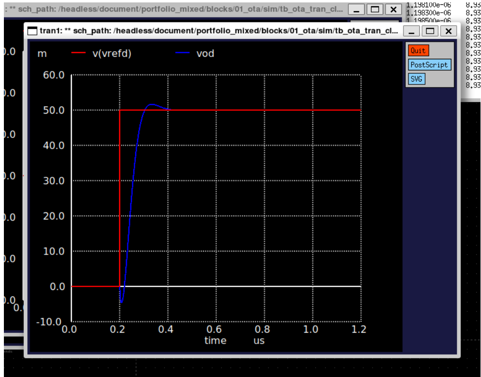
Figure 3: Closed-loop 50 mV differential step response.
