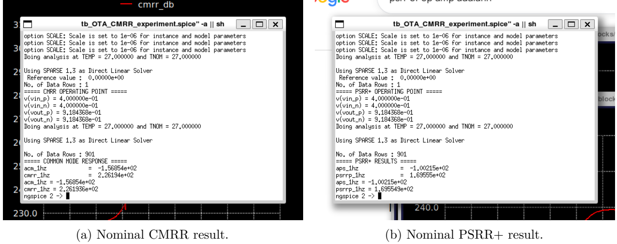
Figure 7: Rejection measurements at the nominal schematic level.
