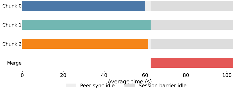
QMSum 3-way fan-in workflow node timing (n=60)
