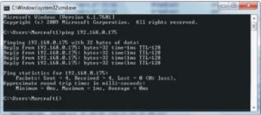
FIGURE 23.14 Ping
