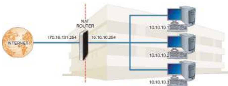
FIGURE 20.1 NAT Configuration
