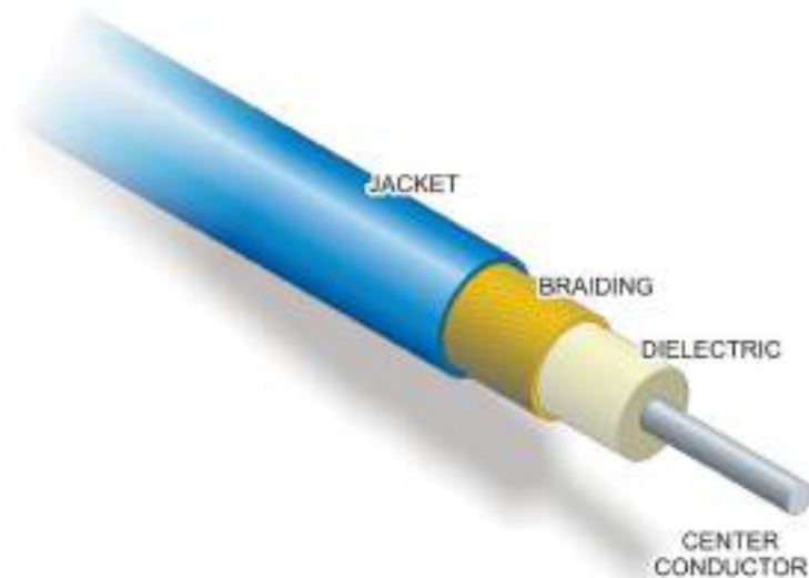
FIGURE 16.2 Coaxial Cable
