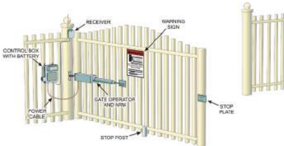
FIGURE 2.9 Swinging Gate
