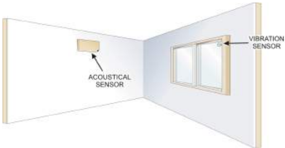
FIGURE 4.7 Glass-Breakage Sensors
