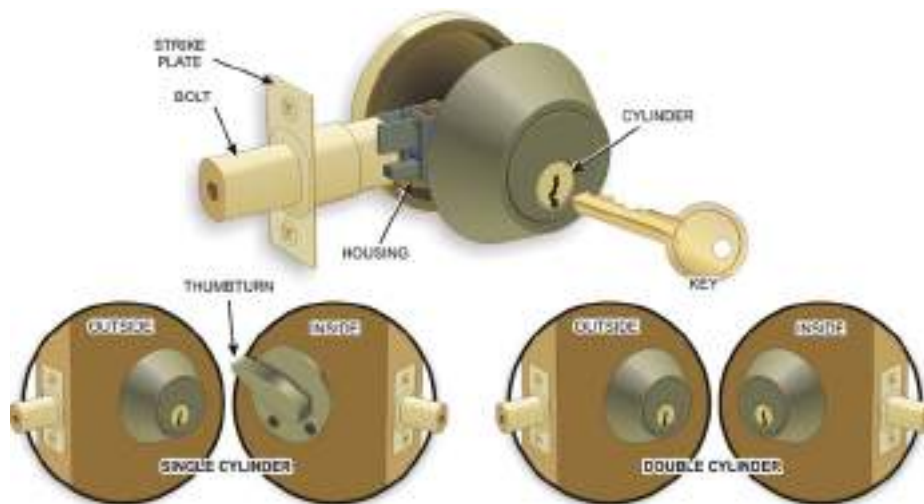
FIGURE 2.5 Key-Locking Deadbolt
