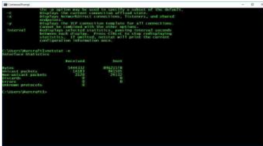
FIGURE 13.12 Observing Data Packet Statistical Information
