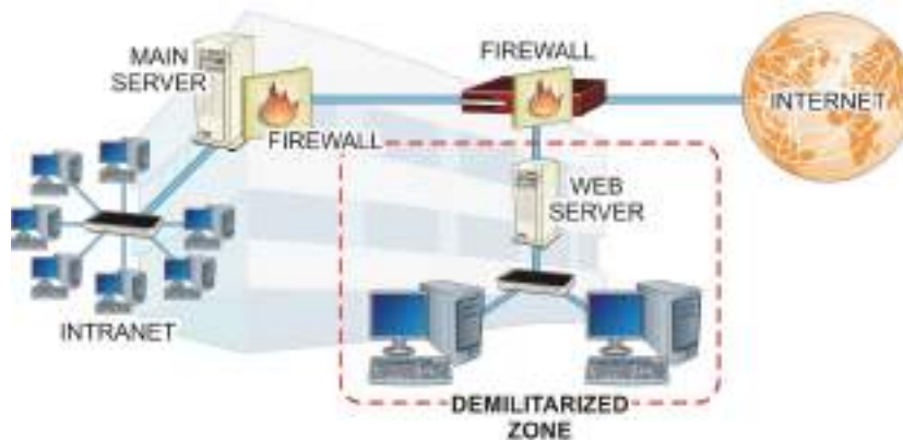
FIGURE 21.10 ADMZ
