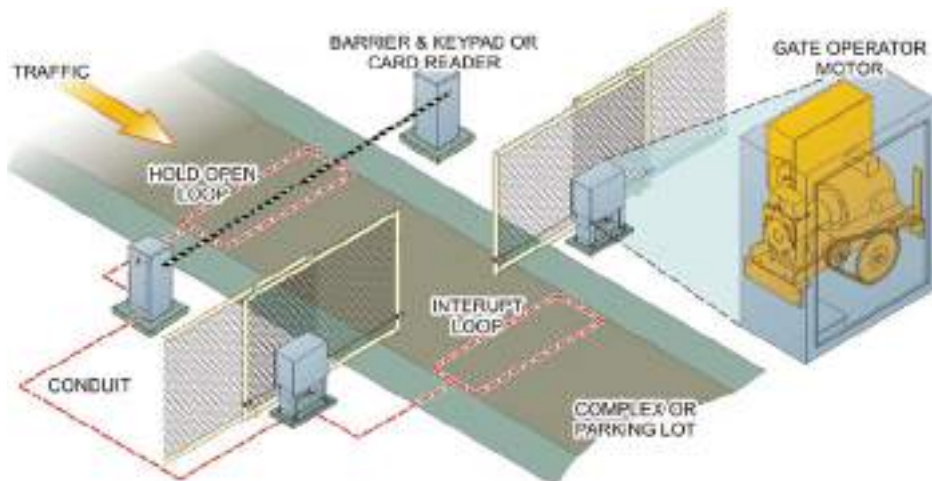
FIGURE 2.8 Sliding Gate
