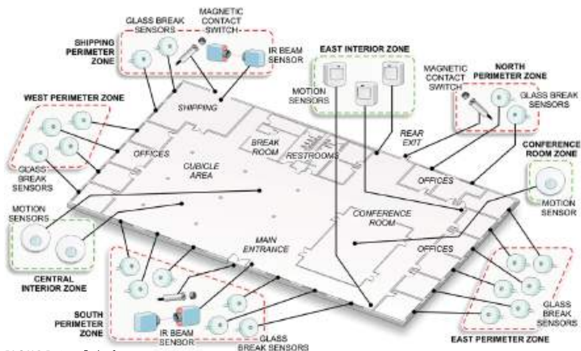
FIGURE 4.5 Zoning Concepts
