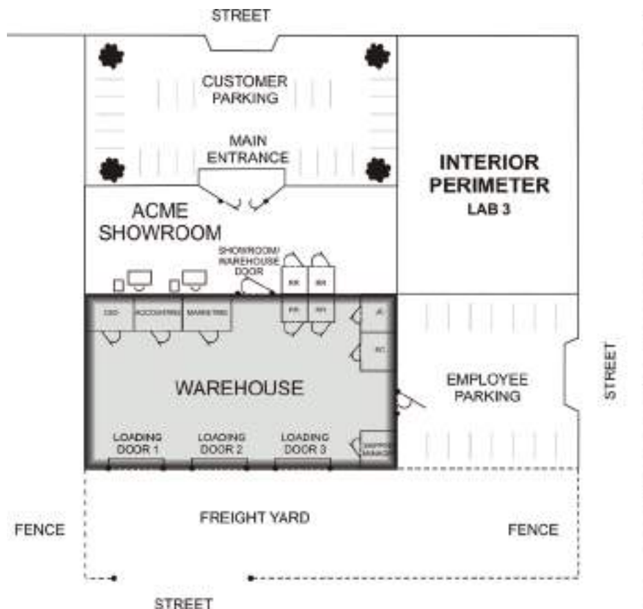
FIGURE 4.18 The Interior Security Zone
