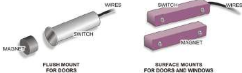
FIGURE 2.17 Window Sensor with Magnetic Switch Contacts
