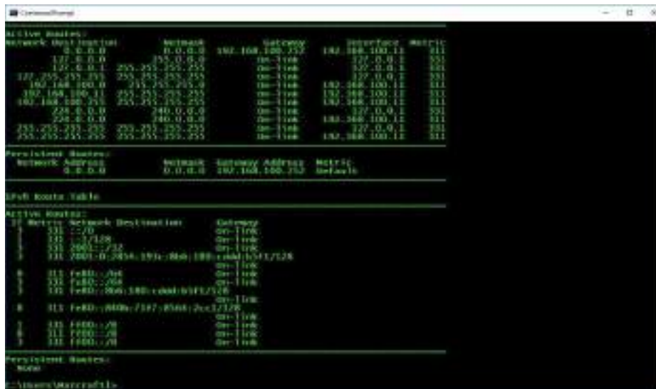
FIGURE 13.13 Displaying the Routing Table
