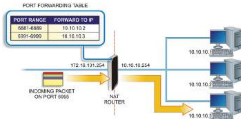
FIGURE 20.3 Port Forwarding
