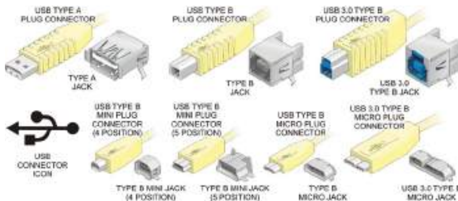
FIGURE 7.10 USB Connectors
