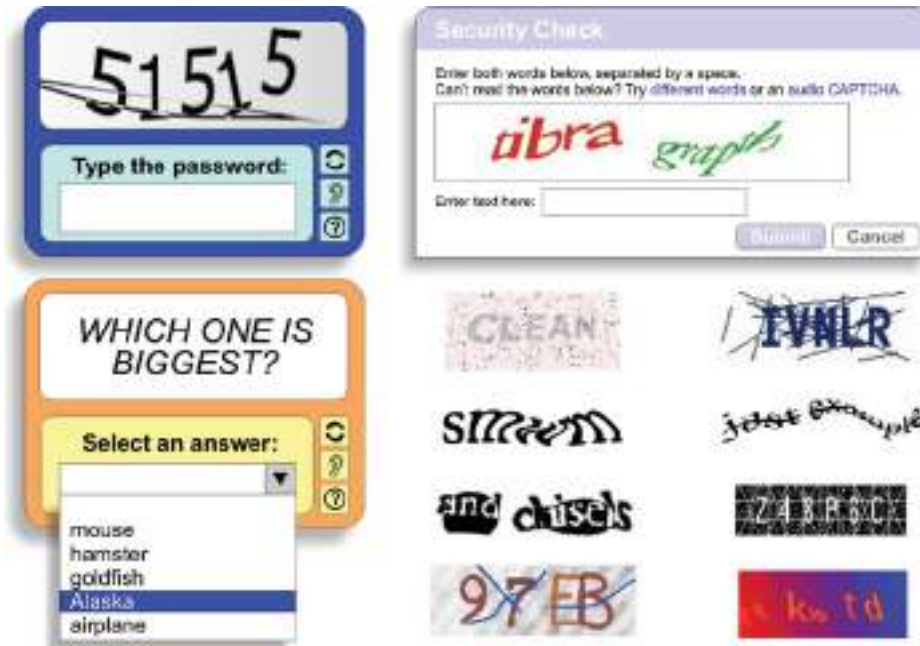
FIGURE 22.5 CAPTCHA Examples
