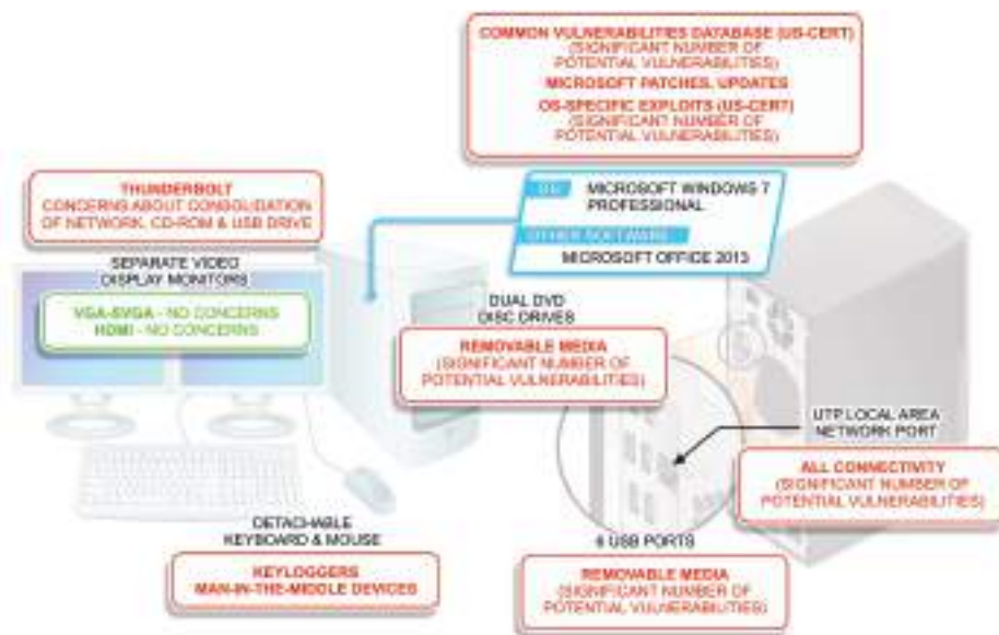
FIGURE 10.2 Known Vulnerabilities
