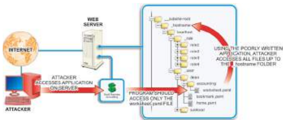
FIGURE 8.5 Directory Traversal
