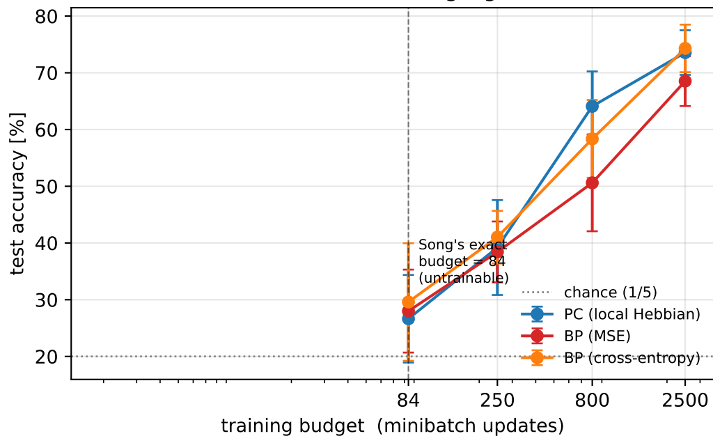
mean of both tasks (Song Fig-4e metric)
