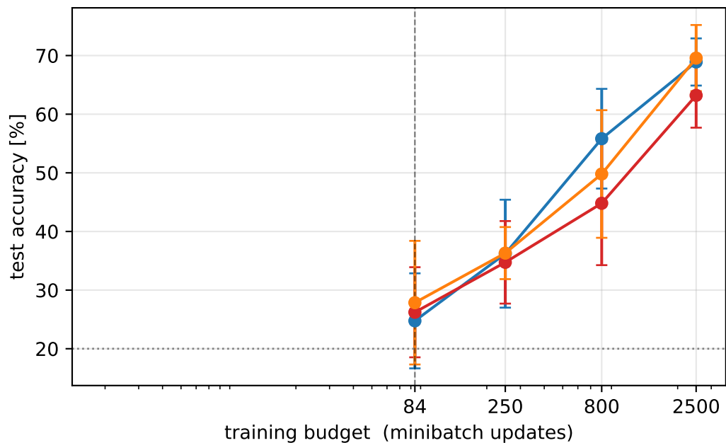
worse task (interference tell)
