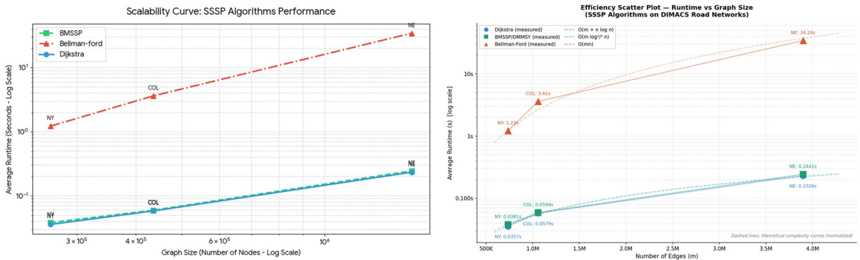
Figure 3. Scalability and efficiency: average runtime against graph size, plus measured points over normalized theoretical trend lines.
