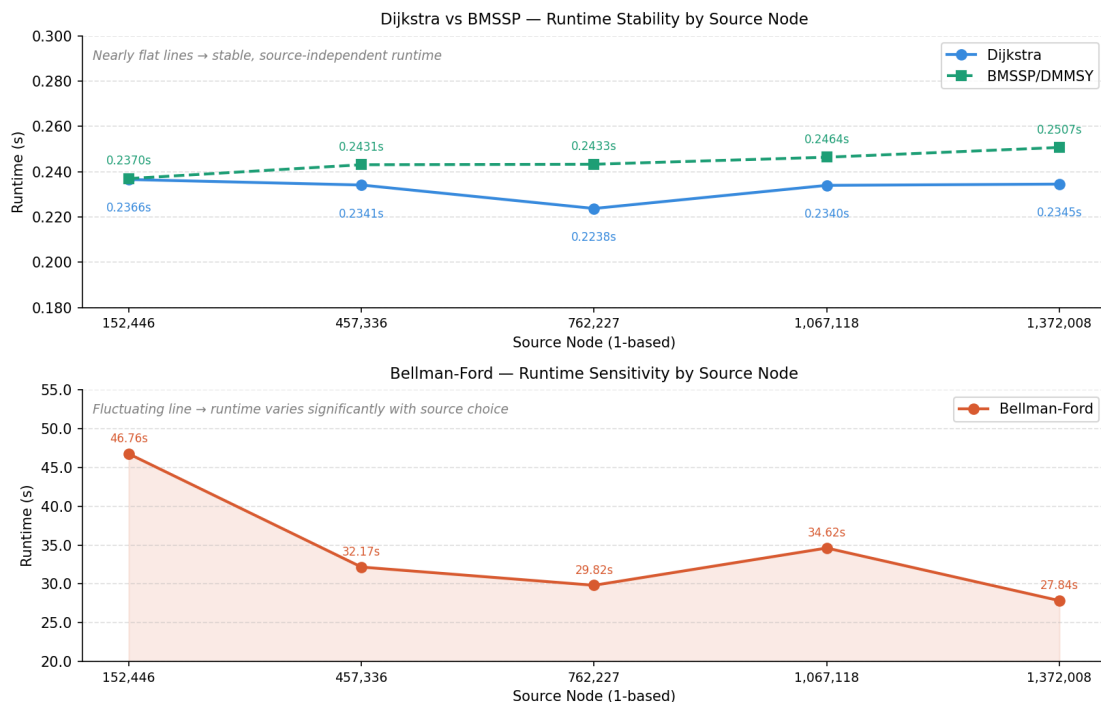
Figure 4. Source sensitivity on NE: Dijkstra and BMSSP remain almost flat, while Bellman-Ford varies strongly with source position.
