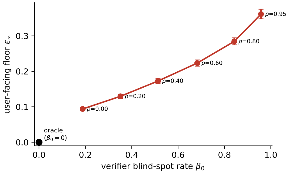
H2: floor scales with \beta_0 ( \pm 1 sd)
