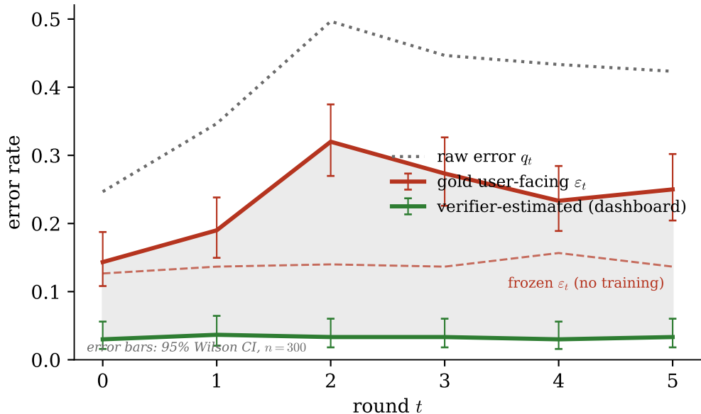
Real LLMs (Qwen2.5-7B, GSM8K): the dashboard is blind
