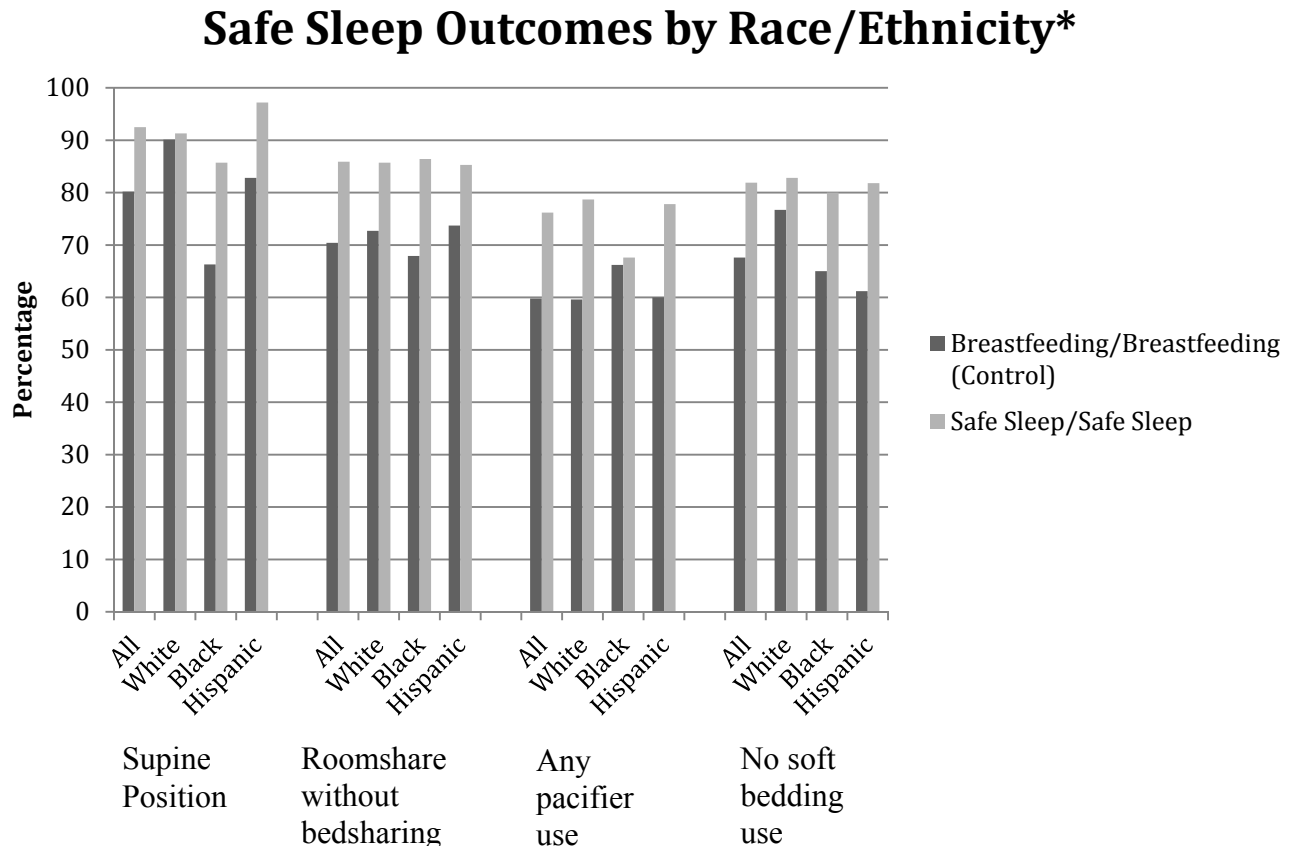
eFigure. Safe sleep outcomes of Breastfeeding Nursing Quality Improvement/Breastfeeding Mobile Health (control) and Safe Sleep Nursing Quality Improvement/Safe Sleep Mobile Health Groups, by race/ethnicity, when infant was >60 days of age
