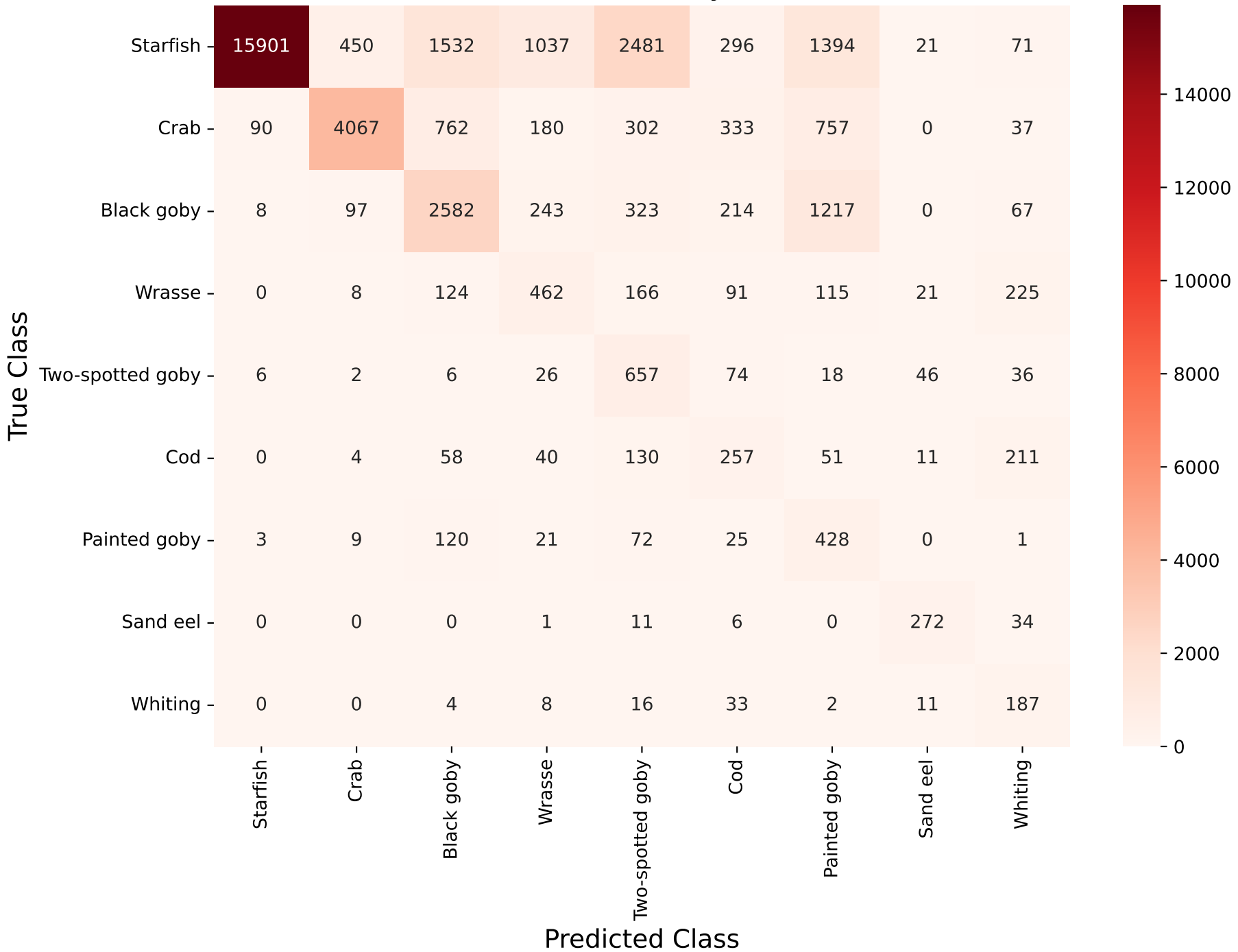
Heat map of DINOv2 embeddings gray normalised median analysis
