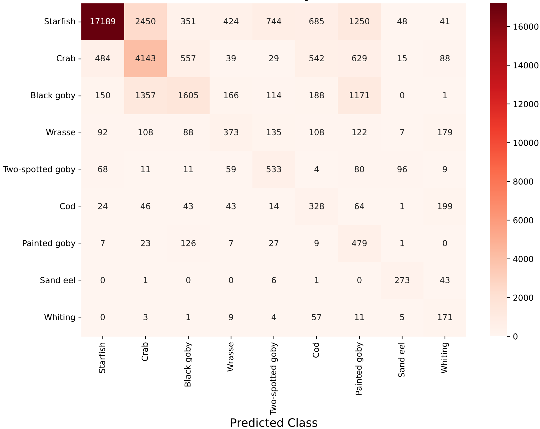
Heat map of resnet embeddings median analysis
