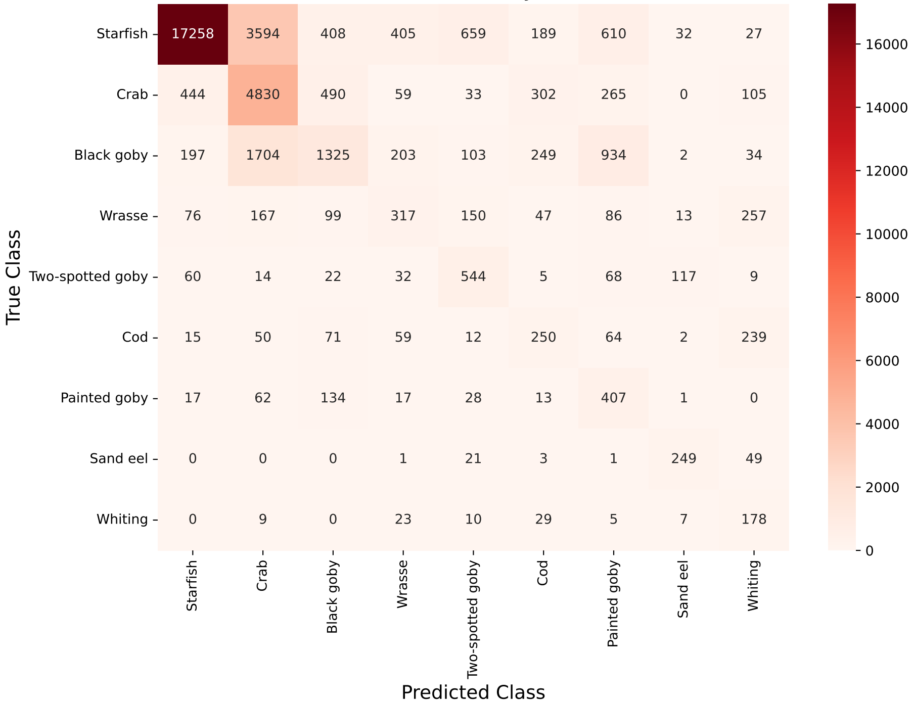
Heat map of resnet embeddings gray normalised median analysis
