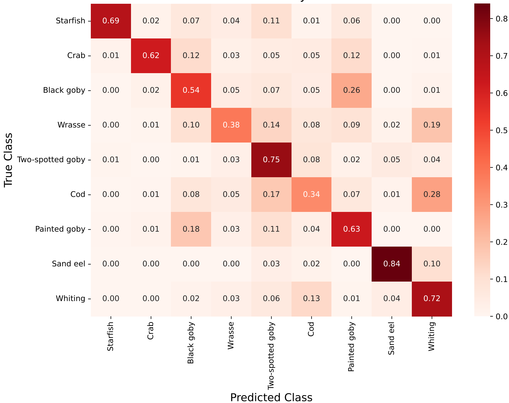
Heat map (row normalised) of DINOv2 embeddings gray normalised median analysis
